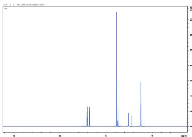
Figure 1: ^1\text{H} NMR of \text{TA}^{\text{OMe}}\text{P}/\text{TFAB} salt.
